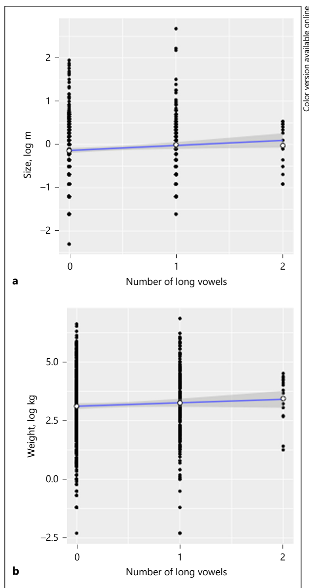
Fig. 14. The effects of long vowels on size (a) and weight (b).
