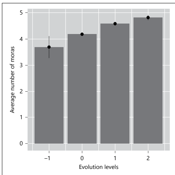
Fig. 7. The average number of mora counts for each evolution level. Pairs that are potentially related by (quasi-)morphological derivation are eliminated. The total number is 322.
