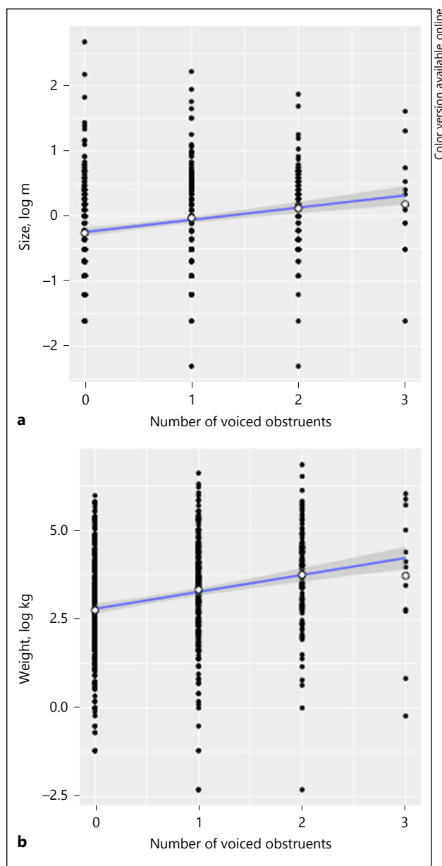
Fig. 4. The effects of voiced obstruents on size (a) and weight (b). The size and weight values are log-transformed (the base = e). The linear regression line is superimposed, with the shaded area representing the 95% confidence intervals. The means in each condition are shown as white dots. The strengths and significance of the linear correlation are tested by a non-parametric Spearman rank-based correlation test.
